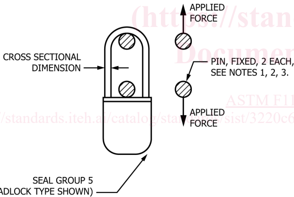
FIG. 4 Schematic Drawings of Pull (Tensile) Test Fixture Requirements for Group 5
