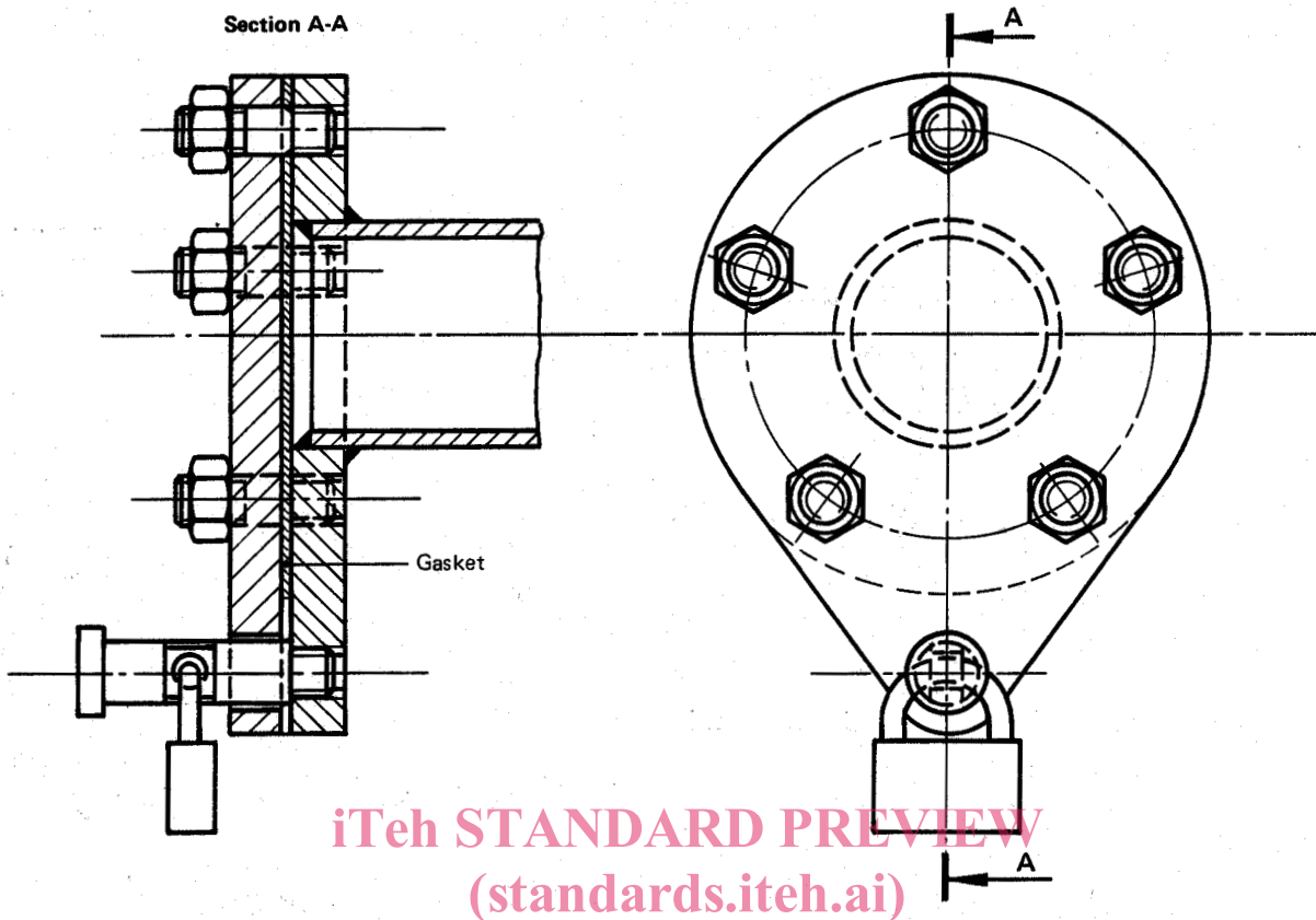
ISO 5620-1978 FIGURE 4 – Flange of ship's piping, with cover closed https://standards.iteh.ai/catalog/standards/sist/1a37b916-480f-4ed7-ac9b-46675893953f/iso-5620-1978
