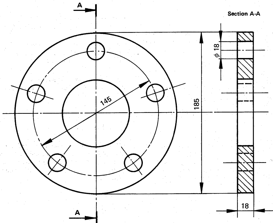
FIGURE 2 - Flange of piping to drinking water supply source
