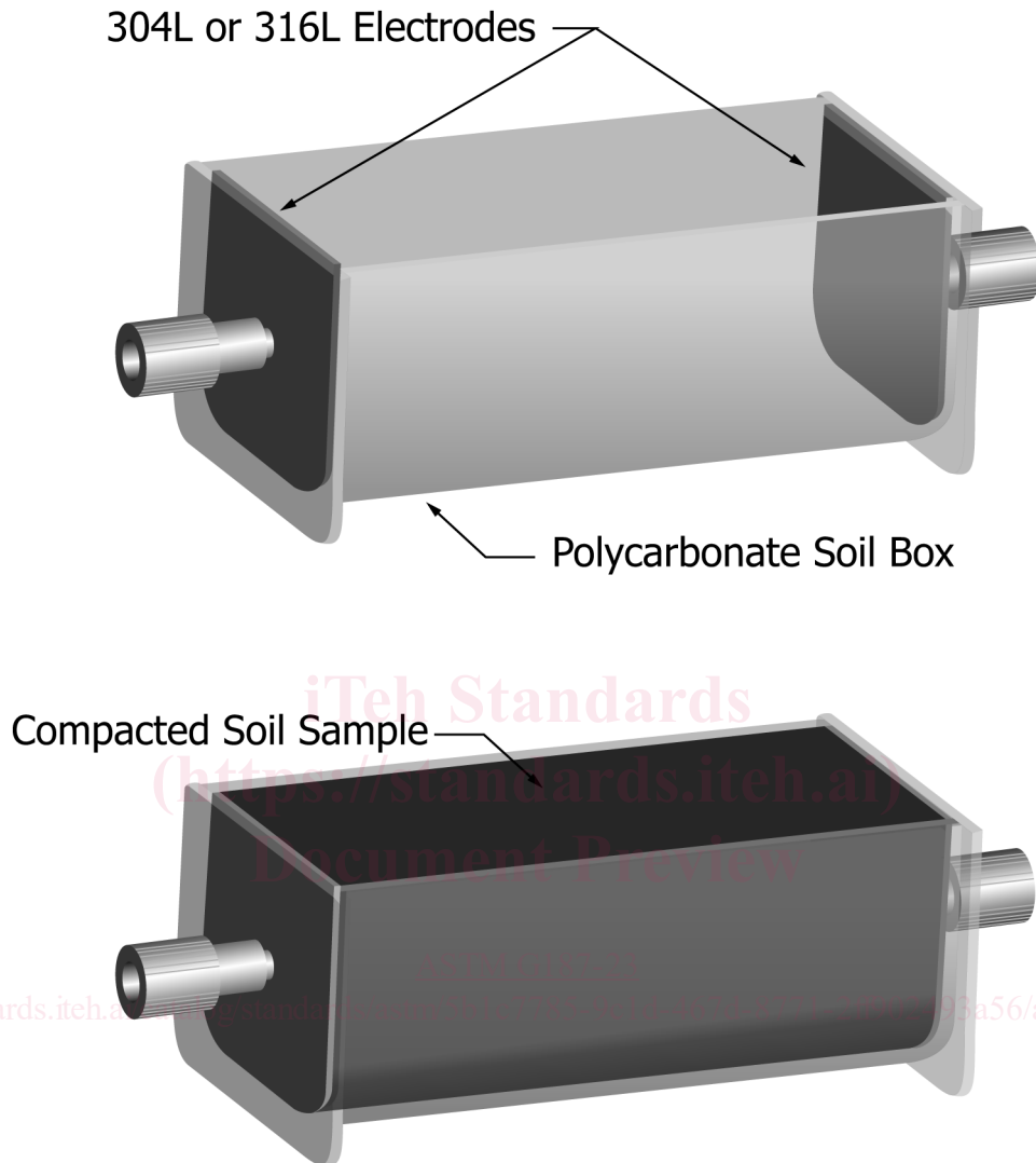
FIG. 2 Typical Two-Electrode Soil Box (Empty and Full)
