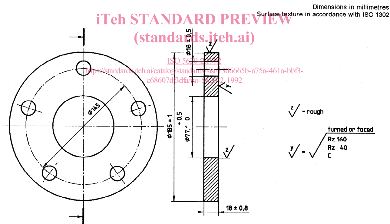
Figure 1 — Dimensions of supply watering flange
