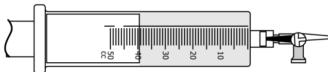
FIG. 4 Oil-Filled Syringe with Handle Towards Syringe
