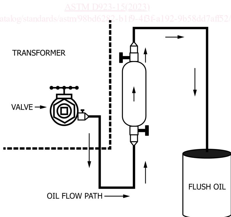
FIG. 5 Sampling with Stainless Steel Sampling Cylinder
