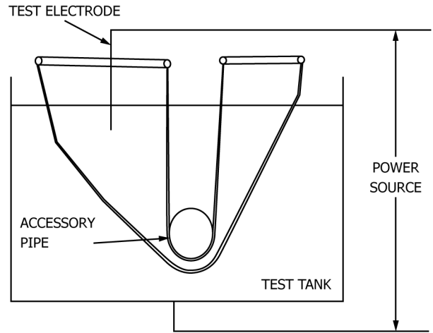
FIG. 4 Water Electrodes, Hammock Mounting
