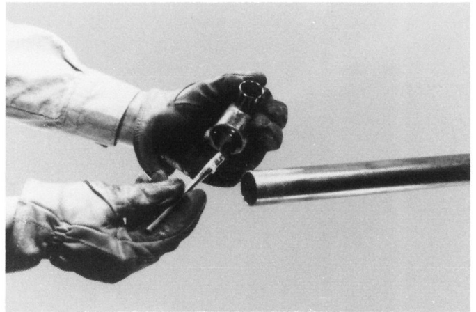
FIG. 11 Fluxing: Fitting
