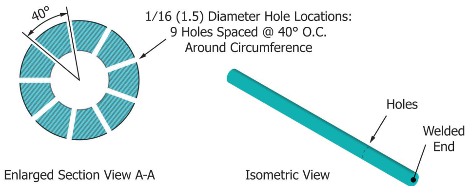
FIG. 3 Tube Type Pressure Sensing Probe
