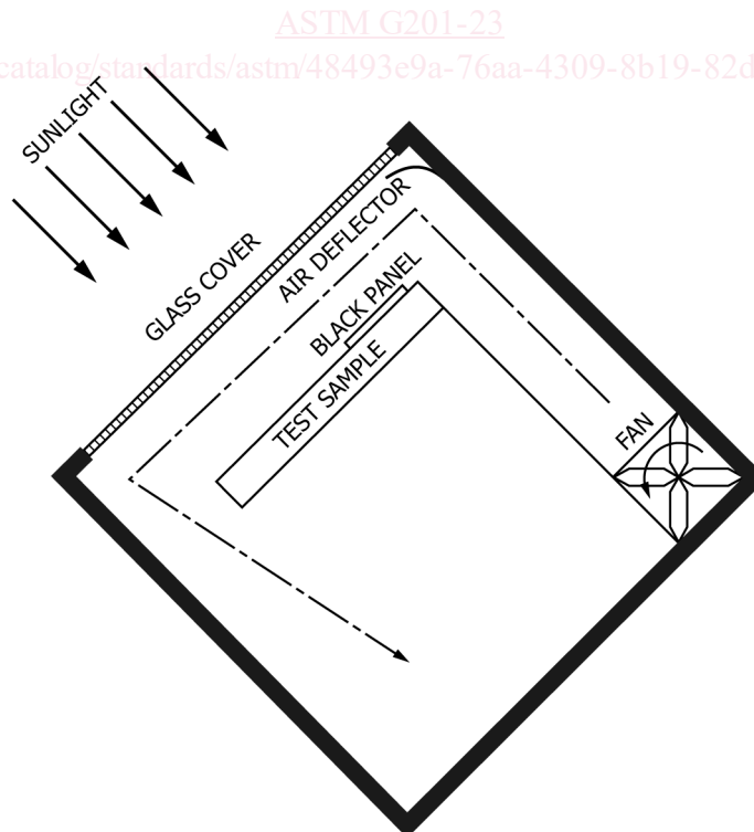
FIG. 1 Diagram of Typical Enclosure with Air Circulation
