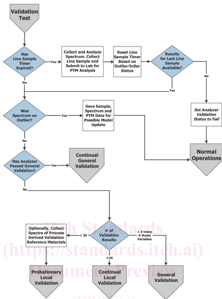
FIG. 3 Flowchart of Process Analyzer Validation Practice Validation Test
