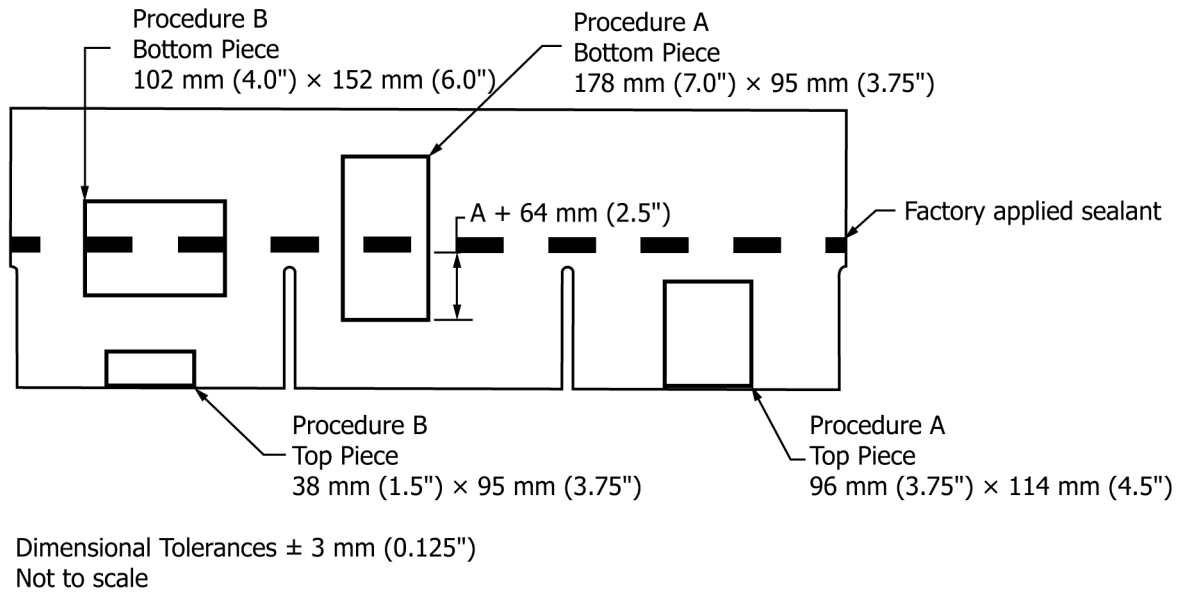
FIG. 5(a) Plan View of Shingle-Layer Shingle Showing Typical Specimen Locations
