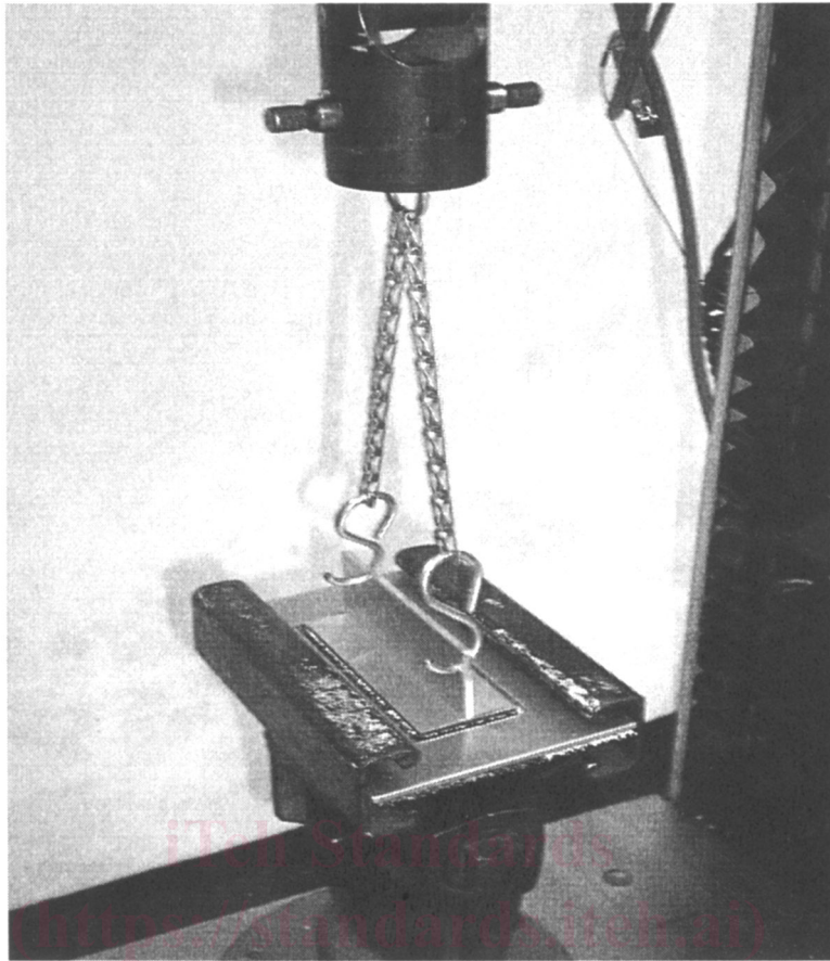
FIG. 4 Shingle Uplift Test Apparatus—Procedure B
