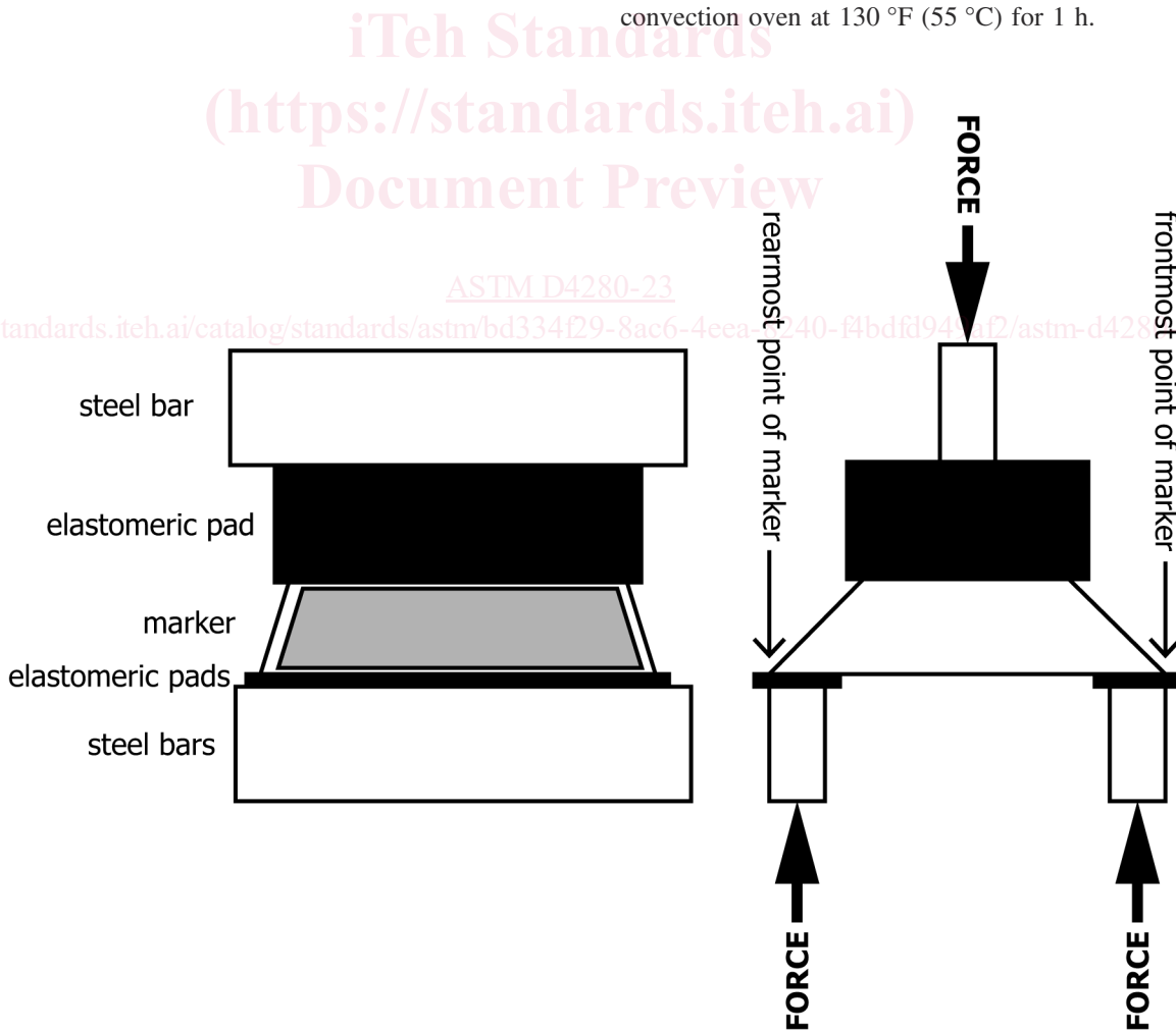
FIG. 4 Longitudinal Flexural Strength Test
