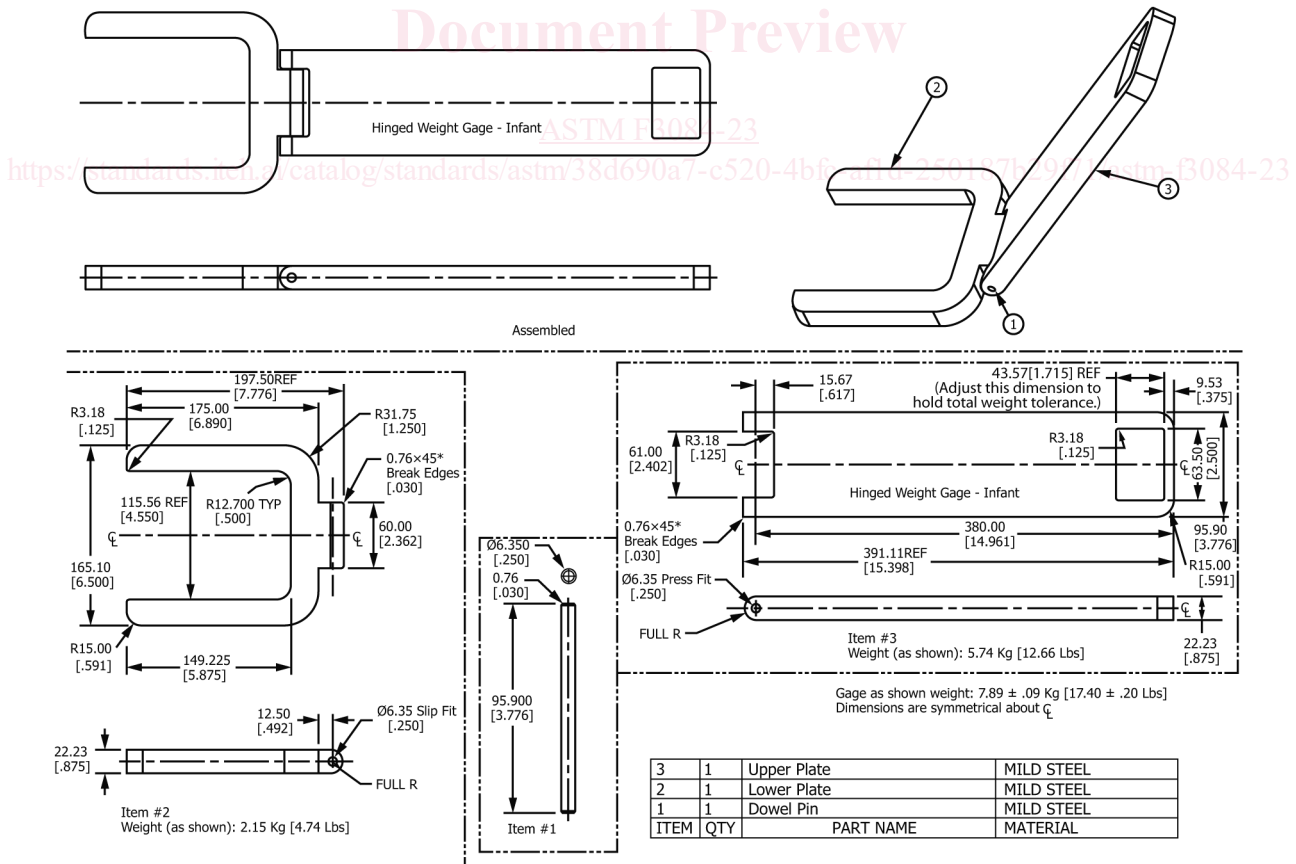
FIG. 6 Hinged Weight Gauge—Infant
