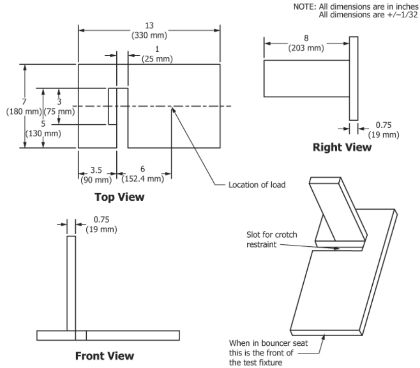
FIG. 8 Forward Stability Test Fixture
