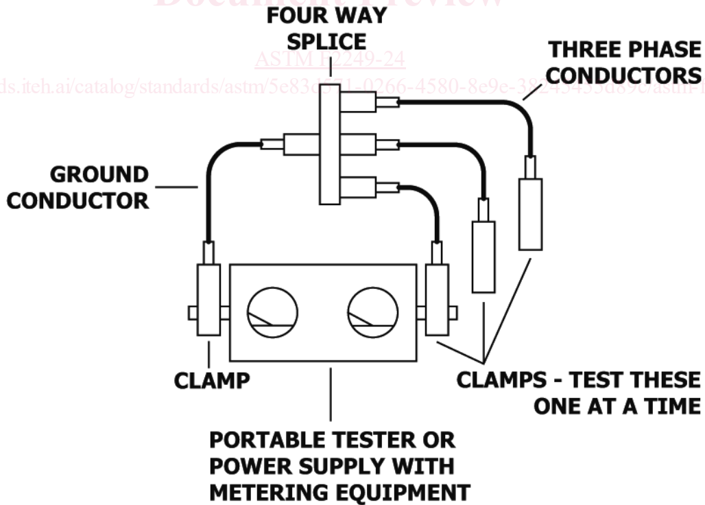
FIG. 2 Typical Configurations
