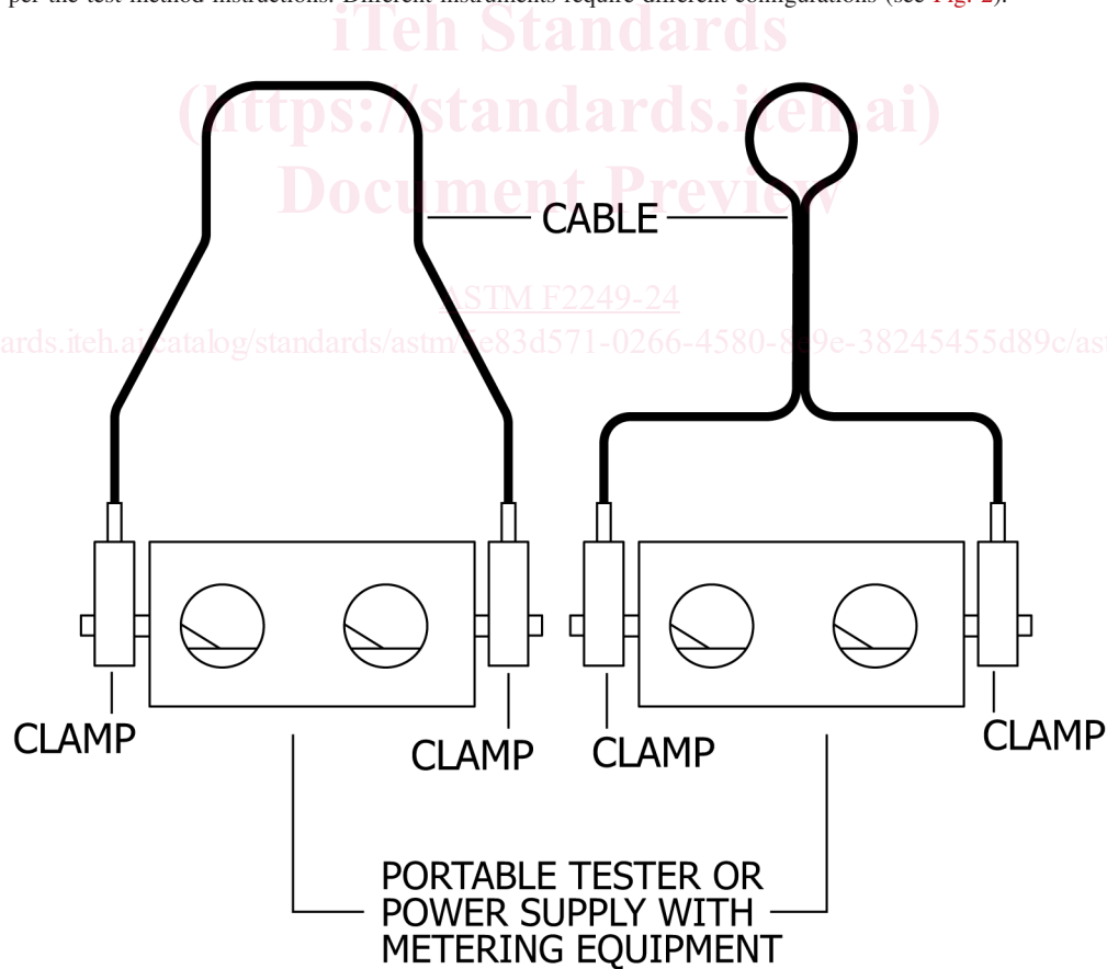
FIG. 2 Typical Configurations
