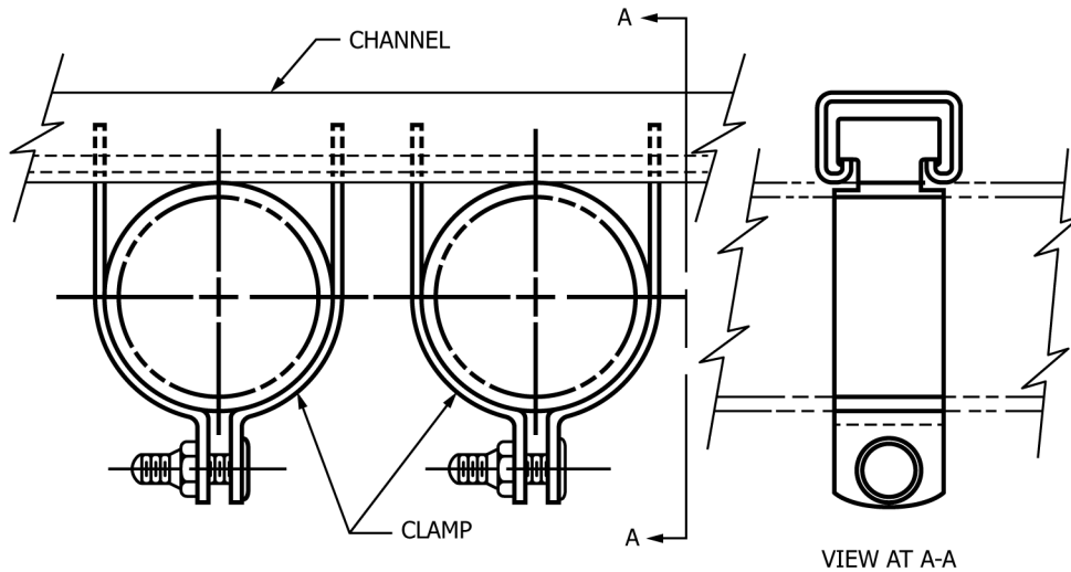
FIG. 7 Clamp Hanger Assembled with Mounting Channel
