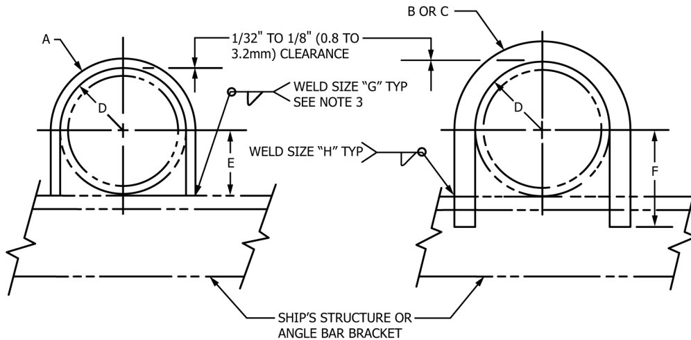
(a) Flat Bar U-Type
