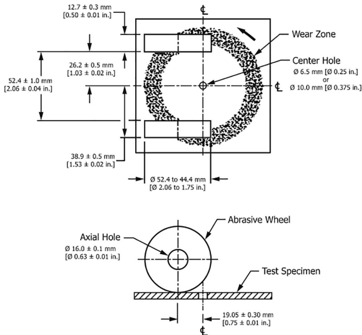
FIG. 2 Arrangement of Rotary Platform Abraser Test Set-up
