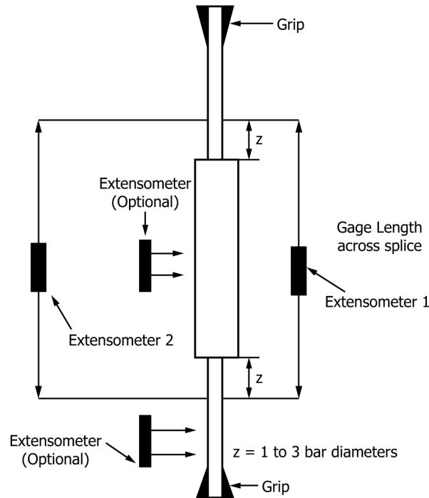
FIG. 1 Specimen Set-up and Gage Gauge Length
