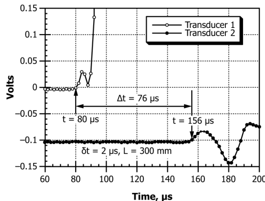
FIG. 2 Example of Waveforms Obtained Using Procedure A (Only Early Part of Waveforms Are Plotted)
