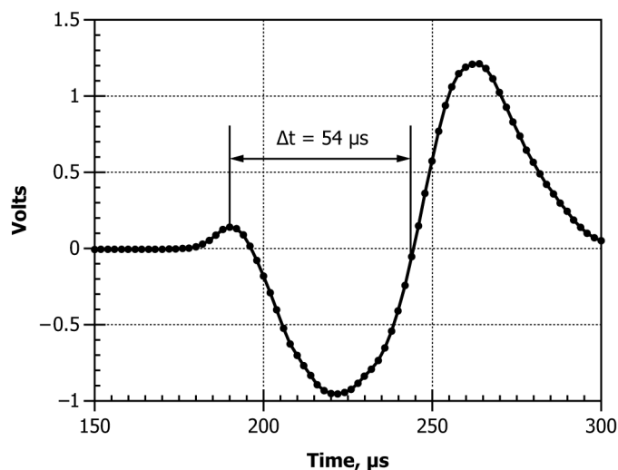
FIG. 3 Expanded View of Surface-Wave Portion of Waveform Showing Width of Surface Wave Signal as Approximation of Contact Time of Impact
