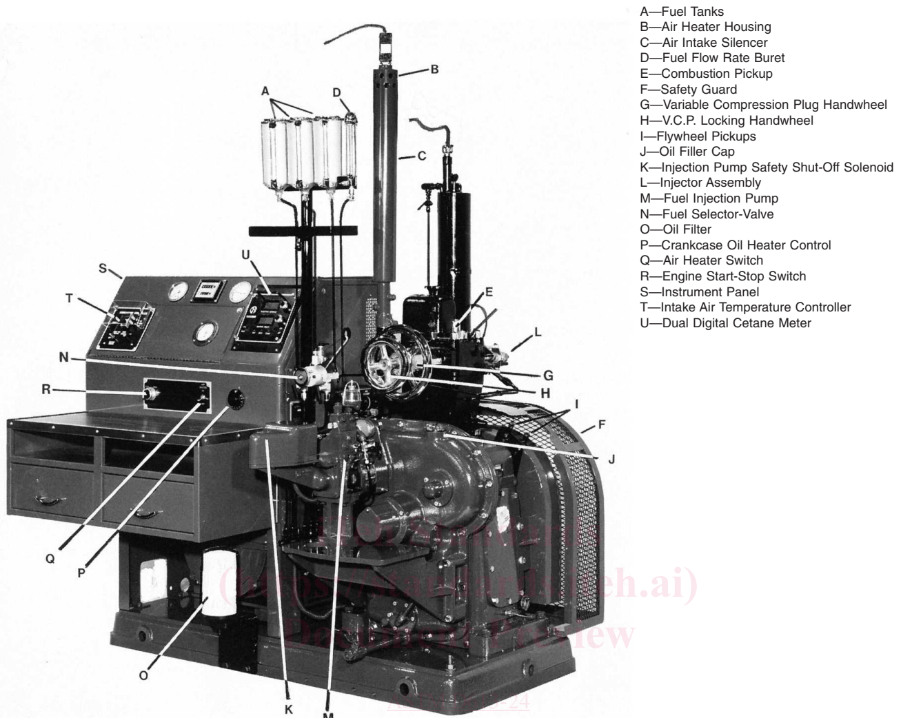
FIG. 1 Cetane Method Test Engine Assembly
