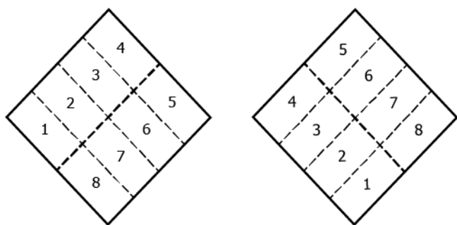
Rounds 1 and 3 Rounds 2 and 4 FIG. 1 Order of Tamping in Molding of Test Specimens
