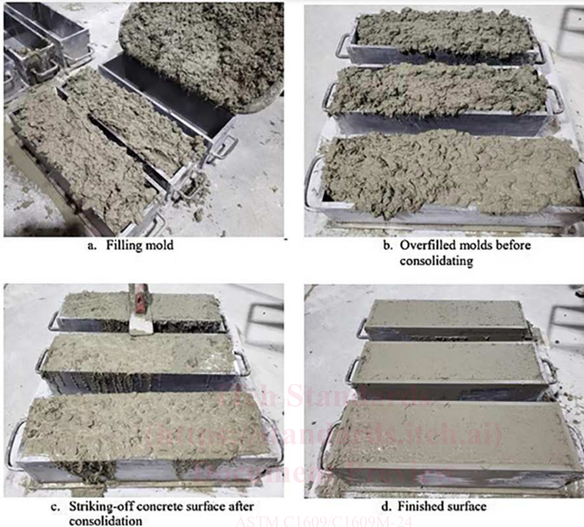
https://standards.iteh.ai/catalog/standards-astm-org/astm-c1609-c1609m-24 FIG. 3 Making Fiber-Reinforced Concrete Test Specimens
