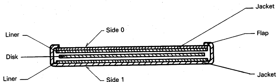
Figure 2 — Section A-A
