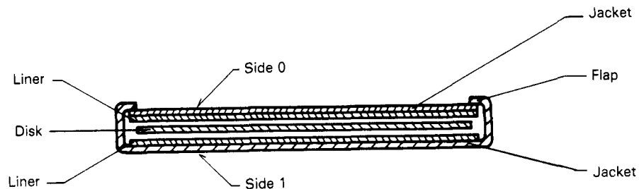
Figure 2 — Section A-A
