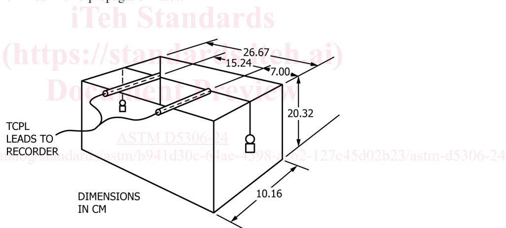
FIG. 1 Apparatus for Determination of Linear Flame Propagation Rates
