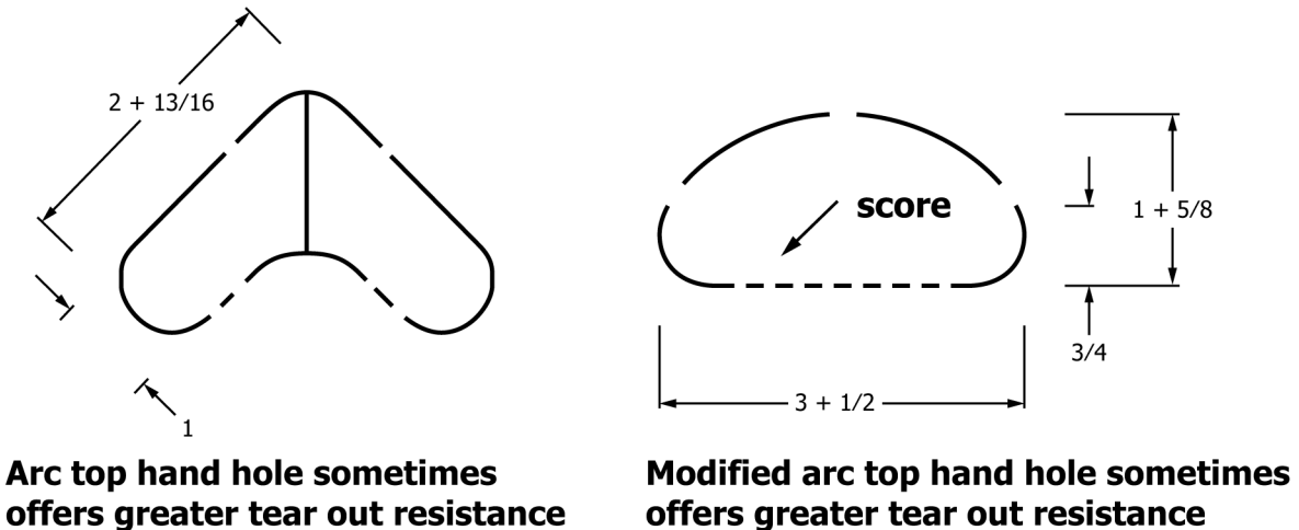
FIG. 1 Common Hand Hole Types
