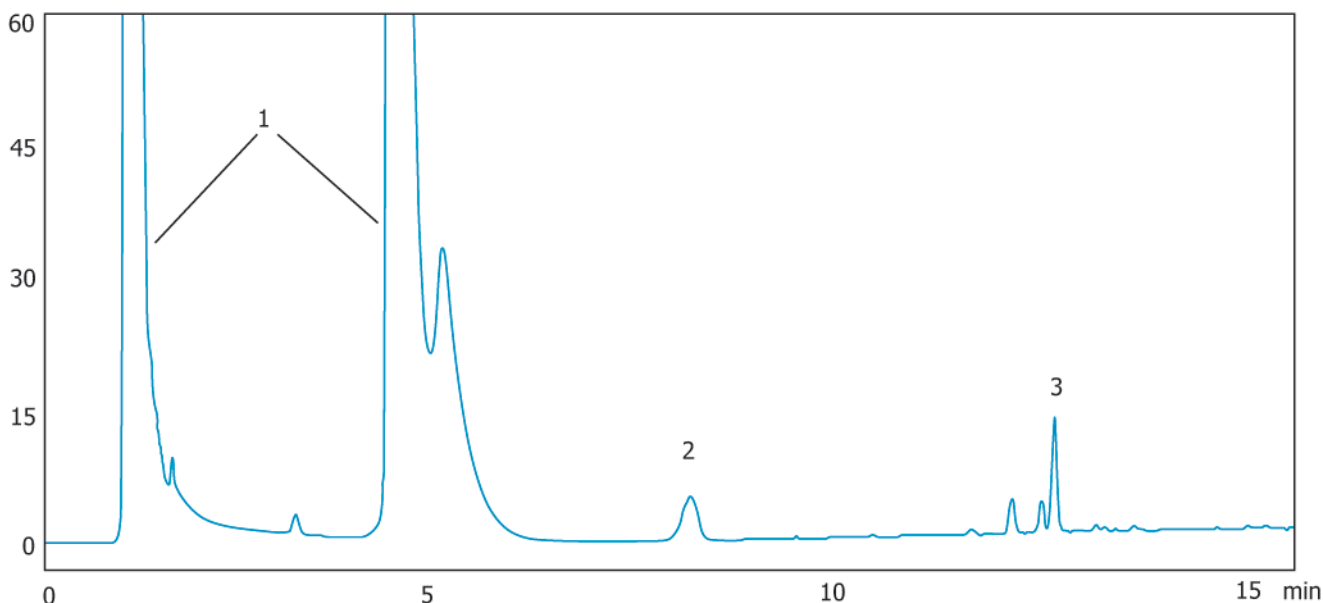
FIG. 2 Chromatogram of a PTA Sample (Reverse Phase HPLC, Gradient Elution Mode) 1-PTA, 2-4-CBA, 3- p -TOL
