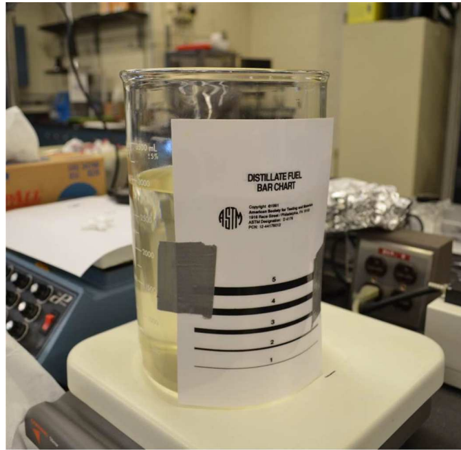
FIG. 3 Taping of Double-Sided Distillate Fuel Bar Chart to 4 L Beaker
