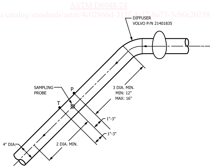
FIG. 2 Exhaust Piping
