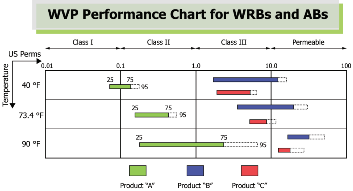
FIG. 1 Proposed WVP Performance Chart for WRB/AB
