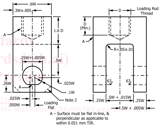
FIG. 1 Typical Configuration of a Dead-Weight Beam Loading Fixture
