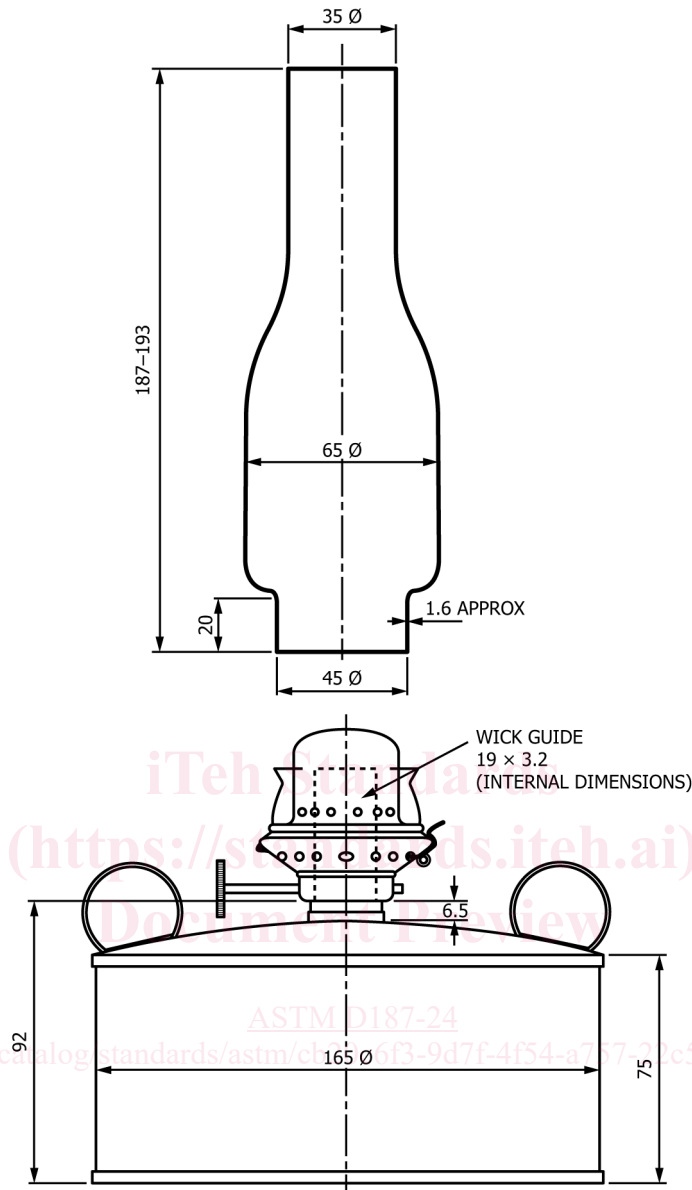
FIG. 1 Test Lamp
