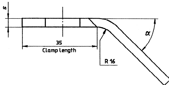
Figure 2 — Bend test
