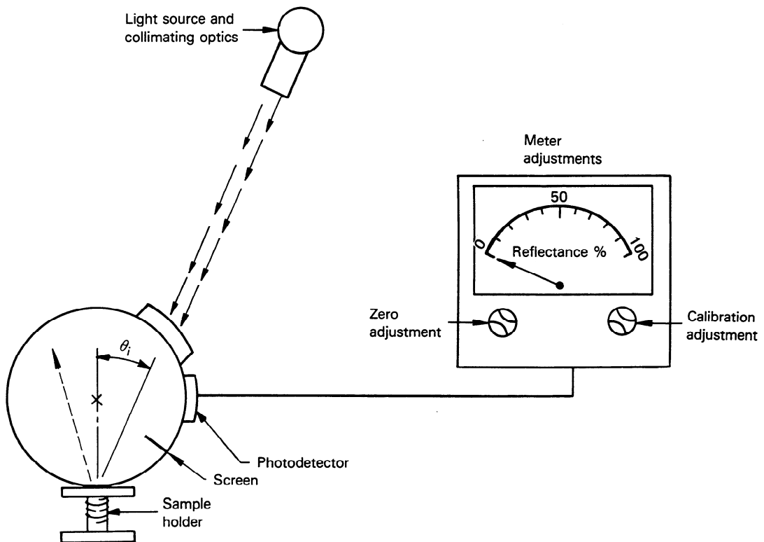
Figure 2 — Generalized reflectometer incorporating an integrating sphere.
