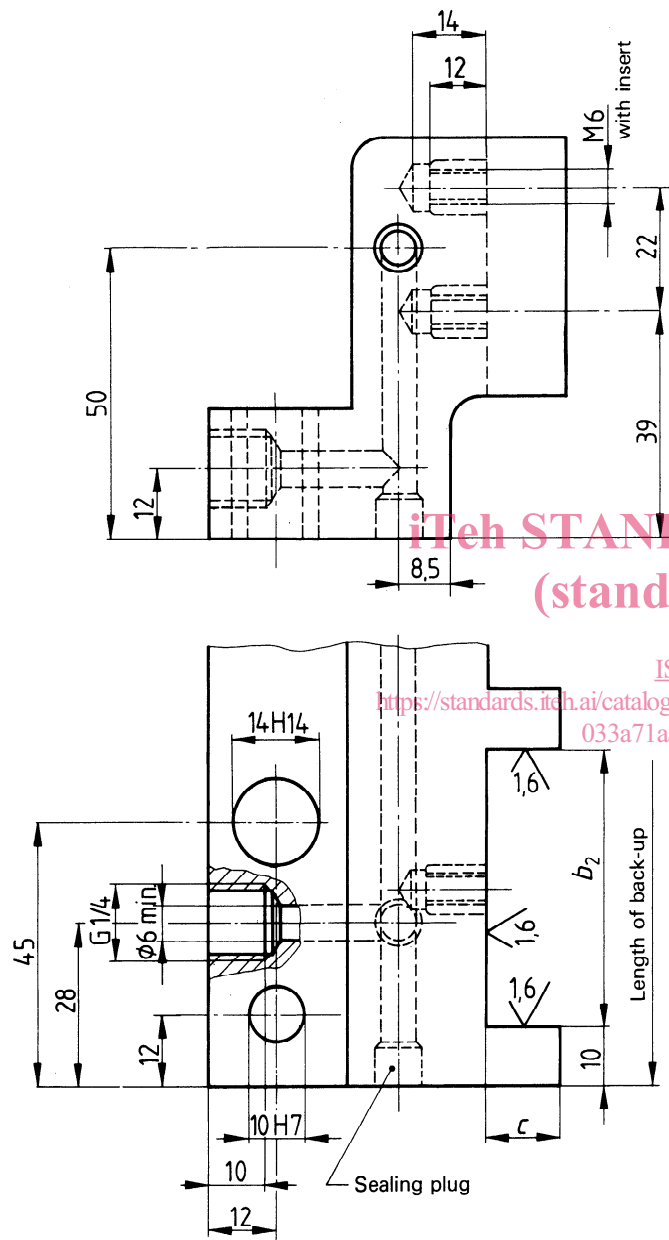
Figure 4 – Dimensions of back-up with cooling holes
