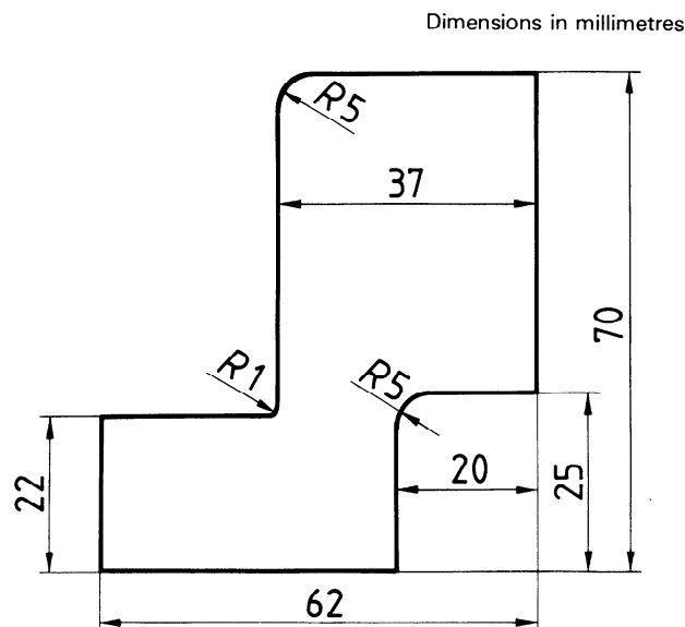
Figure 1 – Dimensions of the back-up profile – Form A
