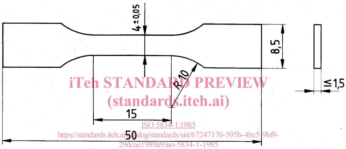
Figure 1 – Specimen
