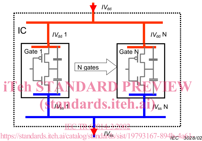
Figure 2 – The basic mechanism for parasitic emission is due to the current driving by all the gates
