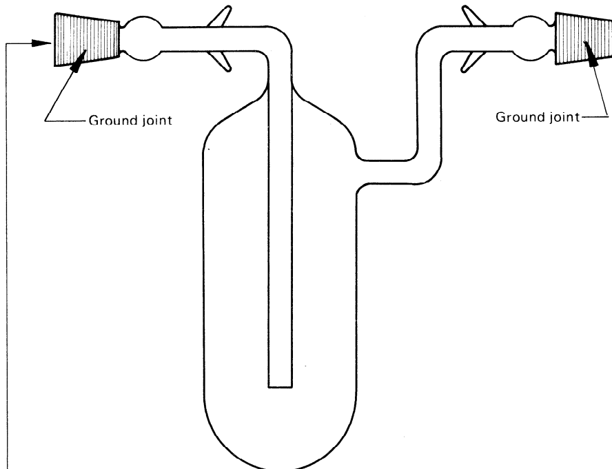
iTeh STANDARD PREVIEW Figure 3 — Liquid trap (6.1.2) (standards.iteh.ai)
