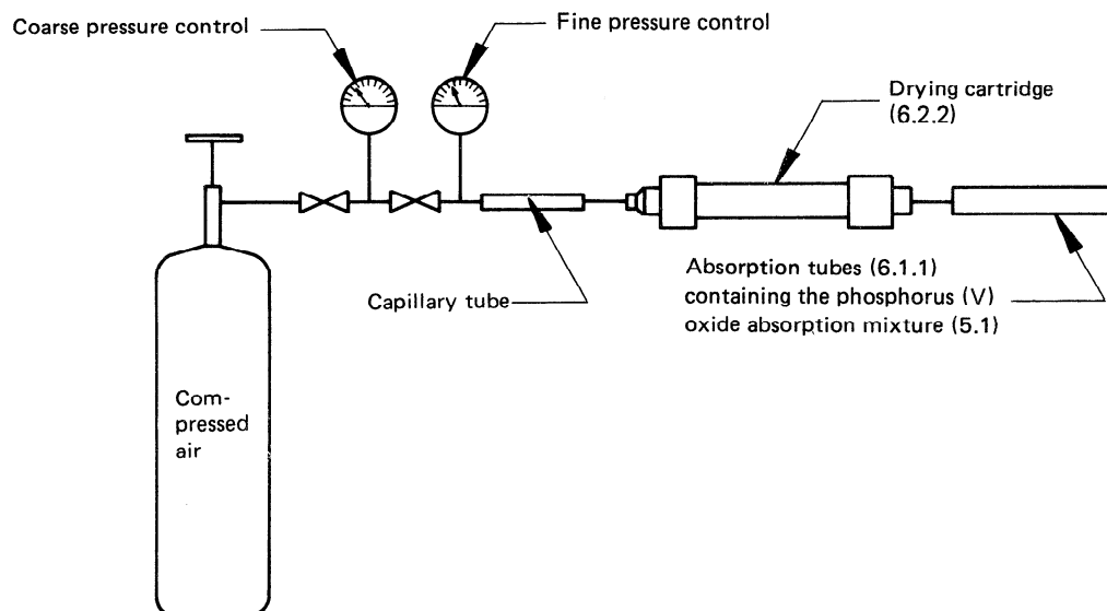
Figure 6 — Scavenging of absorption tubes
