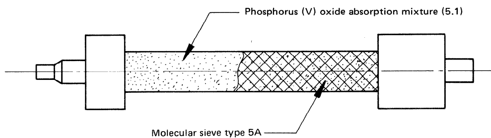
Figure 5 — Drying cartridge (6.2.2)
