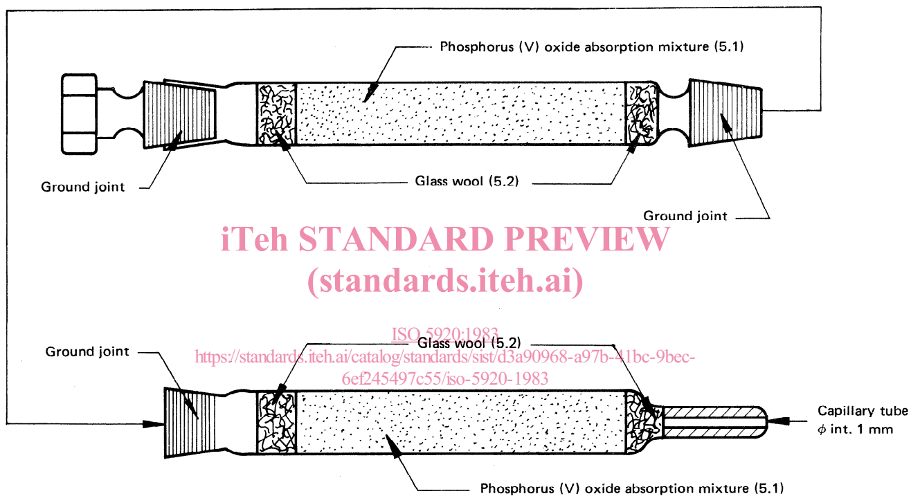
Figure 2 — Absorption tubes (6.1.1)
