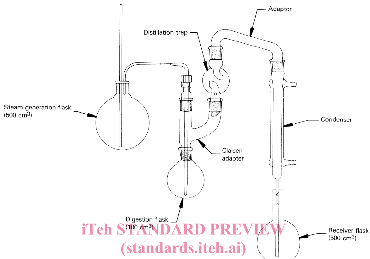
ISO 5945:1989 Figure 1 — Digestion and distillation assembly https://standards.iteh.ai/catalog/standards/sist/561150ae-d656-48d0-959a-a513396cfb57/iso-5945-1989
