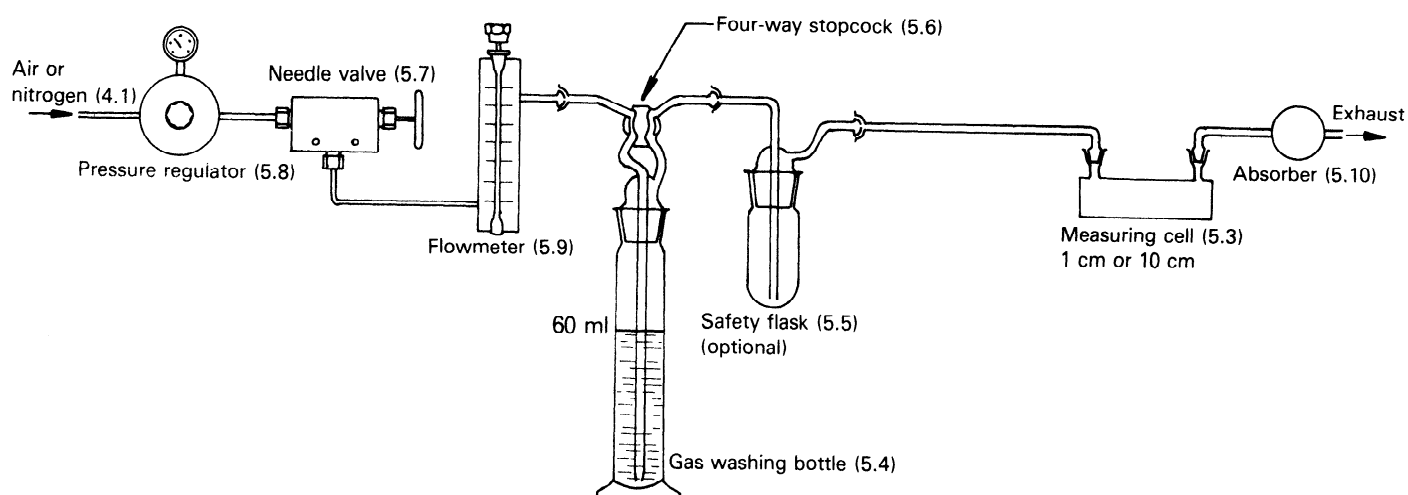
Figure — Typical apparatus for determination of mercury by atomic absorption
