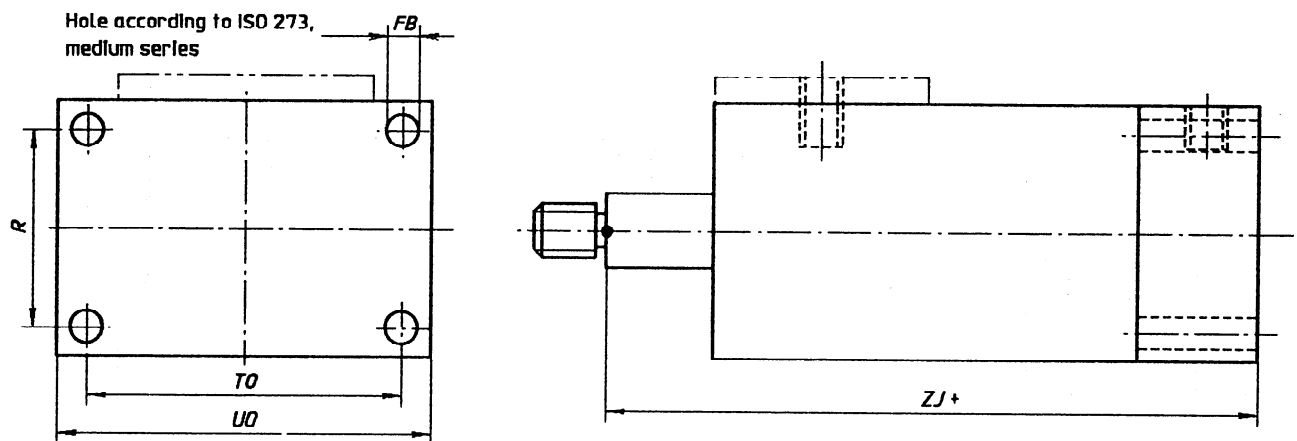
Figure 3 — ME6 — Cap mounting, rectangular
