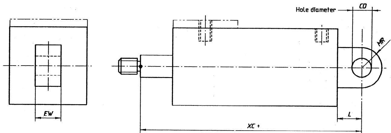
Figure 5 — MP3 — Cap mounting, fixed eye
