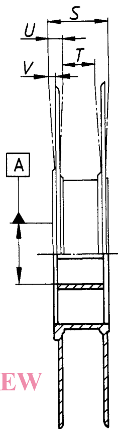
Figure 3 — Maximum lateral runout
