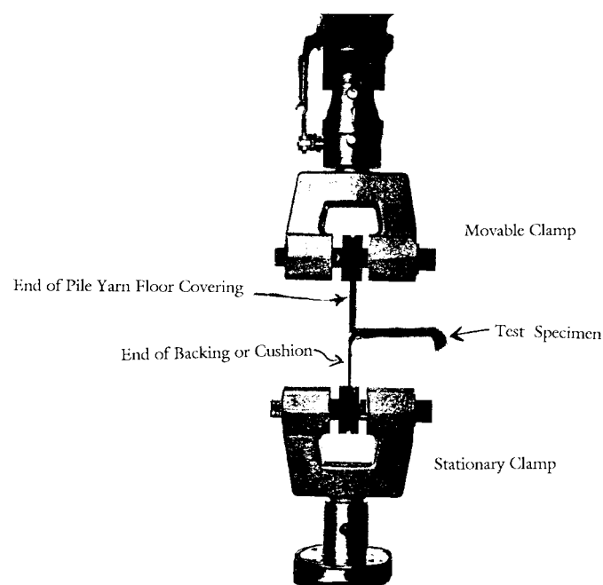
FIG. 1 Specimen Mounted in Clamps
