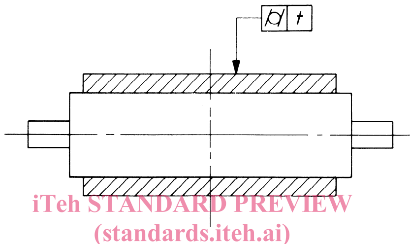
Figure 2 — Cylindricity tolerances
