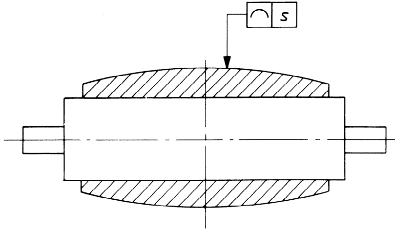
Figure 3 – Crown tolerances
