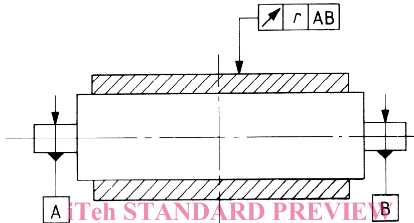
Figure 1 — Run-out tolerances
