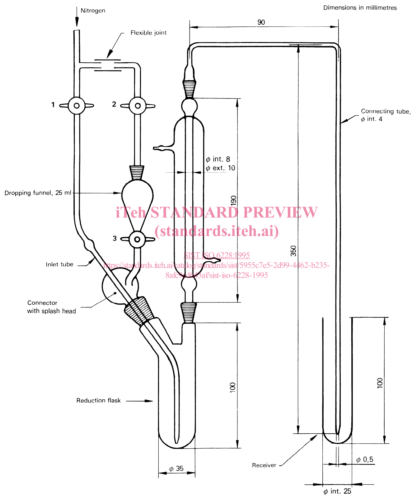
Figure 1 — Typical apparatus for reduction and entrainment
