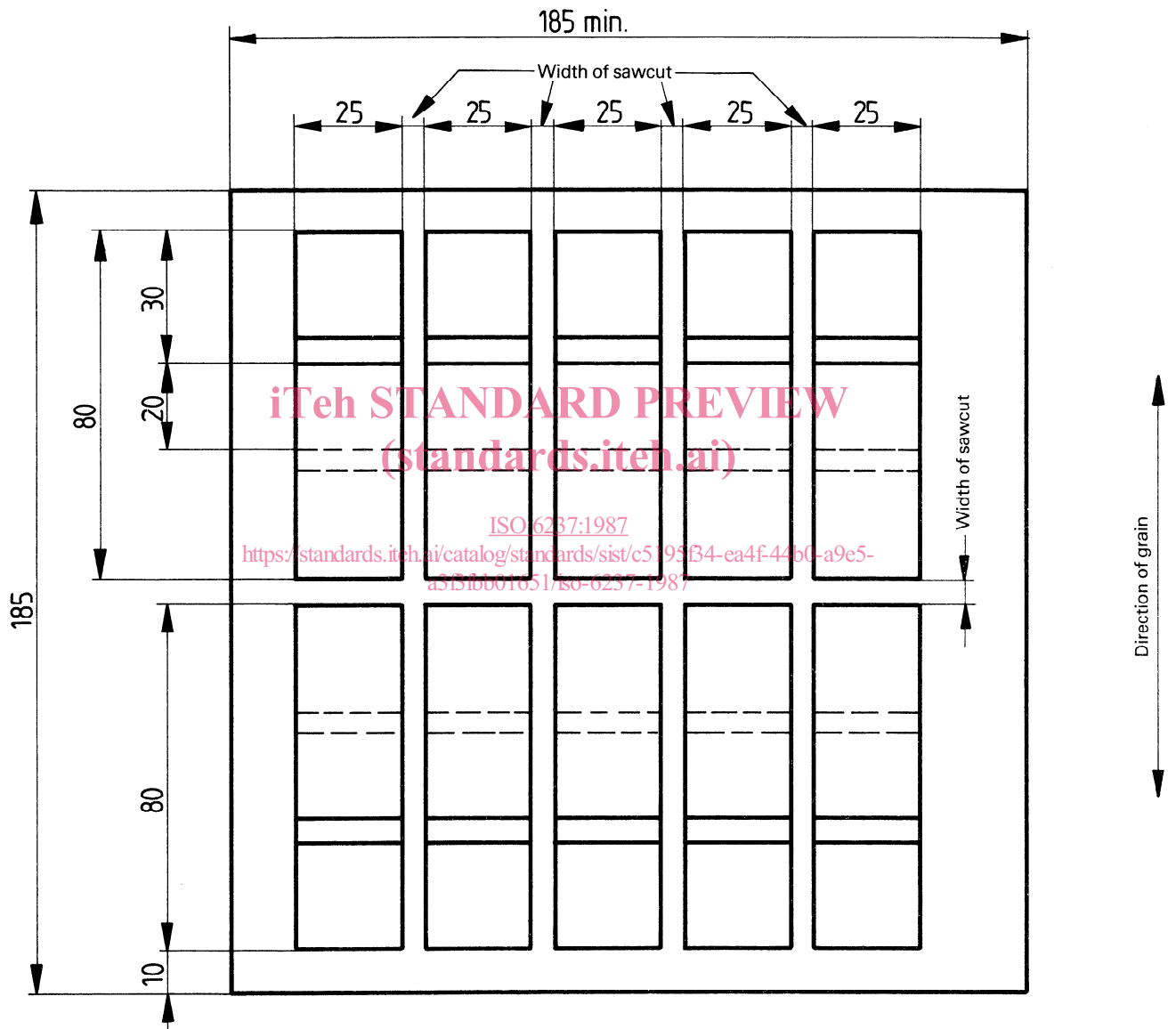
Figure 2 — Suggested arrangement of specimens
