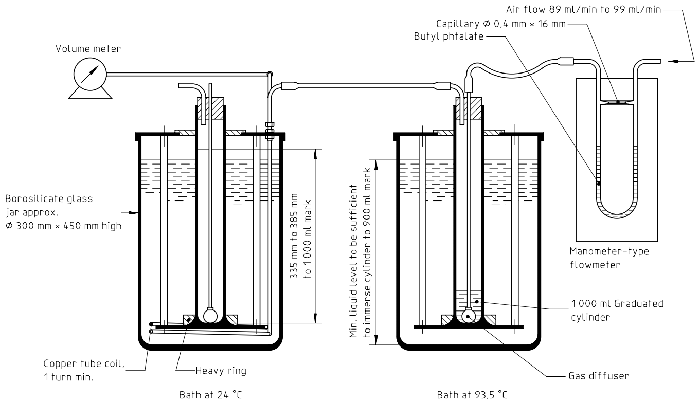
Figure 1 — Foaming test apparatus (standards.iteh.ai)
