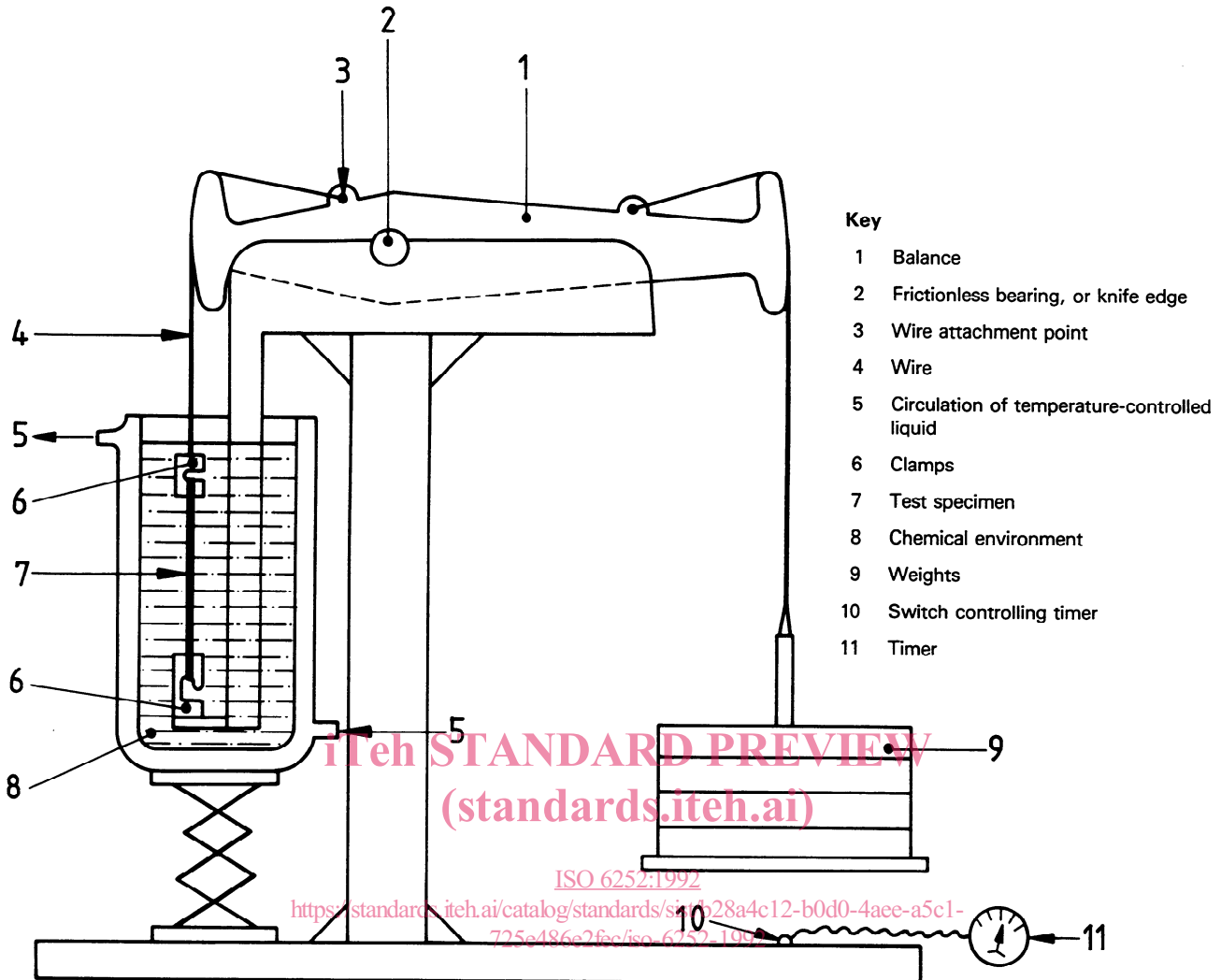
Figure 2 — Balance type of apparatus with 2:1 amplification of load
