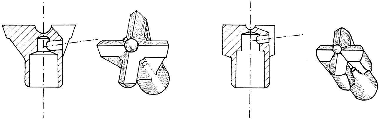
Figure 1 — Typical cutting bits for sampling drill
